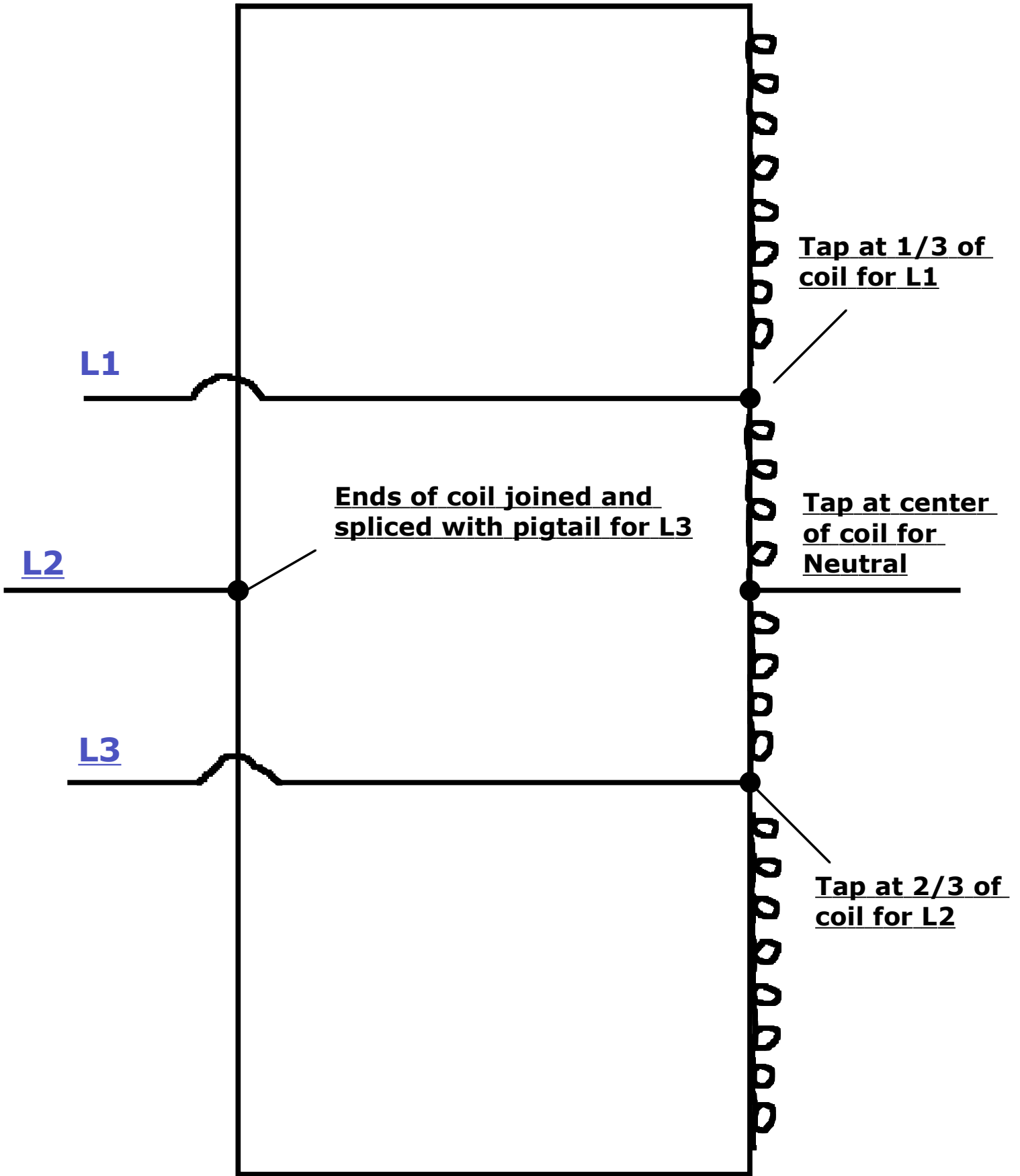
3 Phase Secondary Winding - Delta
