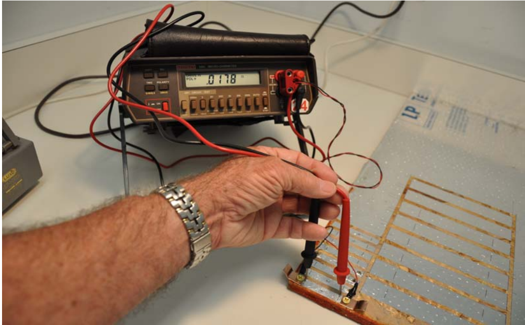
PHOTO # 5 Four Point Measurement of Test Strip Resistance
