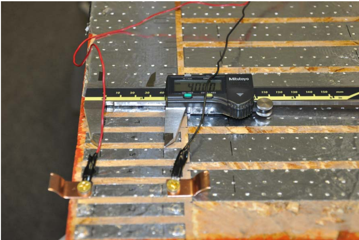
PHOTO # 4 Shows the two sets of sample test strips One set 1cm wide x 4cm long One set 1 inch wide x 4 inches long
