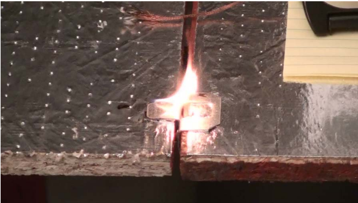
PHOTO #9 Roof Sheathing and Clip Energized With Current of Approximately 50 Amps
