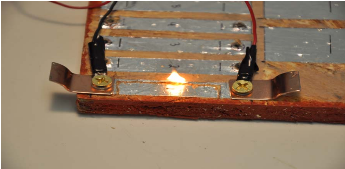
PHOTO #7 Test Strip Ignites at a Current Density of 300 Amps per Square Millimeter
