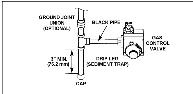
FIGURE 13. GAS PIPING WITH ALL BLACK IRON PIPE TO GAS CONTROL.
