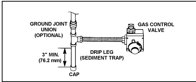
FIGURE 12. GAS PIPING WITH FLEXIBLE CONNECTOR.
